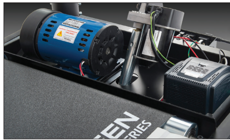
5.0 HP, AC NextGEN III Eco-Drive System™
